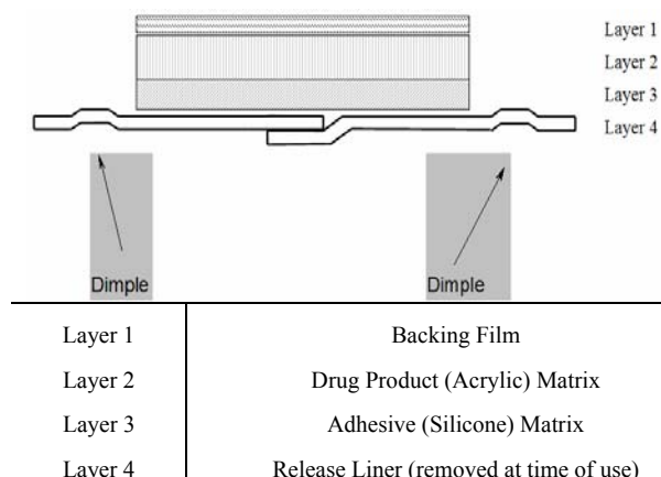
Figure 1: Cross Section of the Patch
